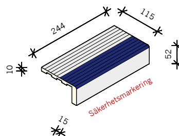
RIBBAD KANTPLATTA C YTA 115x244x10/52 mm
