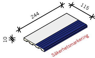
RIBBAD KANTPLATTA C YTA 115x244x10 mm
