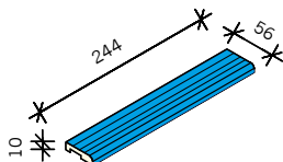
RIBBAD MARKERINGSPLATTA C YTA 150x244x10mm
