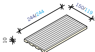
BRED RIBBAD PLATTA C YTA 150x244x10 mm
